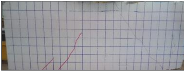
Fig. 6. Crack pattern of reference beam, CB1.
