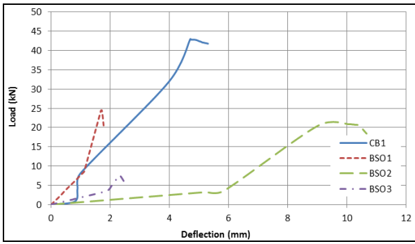
Fig. 5. Comparison of load-deflection curves between reference beam, CB1 and deep beams with square opening BSO1, BSO2, BSO3.
