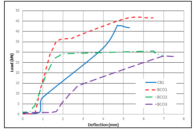
Fig. 4. Comparison of load-deflection curves between reference beam, CB1 and deep beams with circular opening BCO1, BCO2, BCO3.
