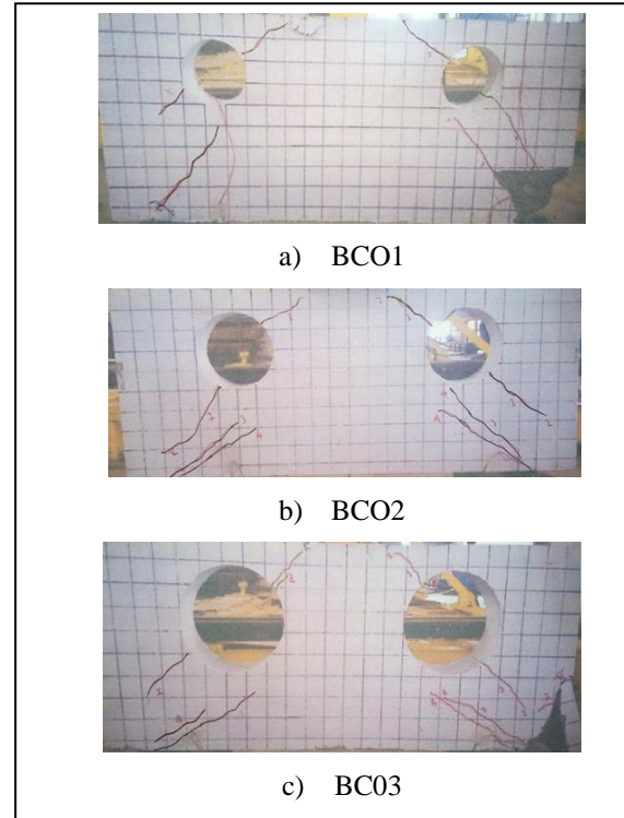
Fig. 7. Crack pattern of RC deep beams with circular openings (a) BCO1 (b) BCO2 (c) BCO3
