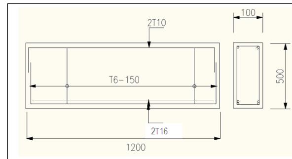
Fig. 3. Schematic diagram of reinforced concrete deep beam.
