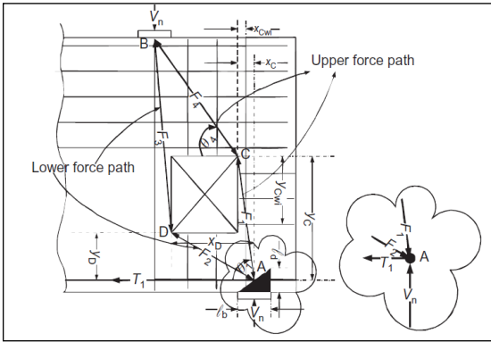
Fig. 1. Load paths of deep beams with web openings [5], [6]
