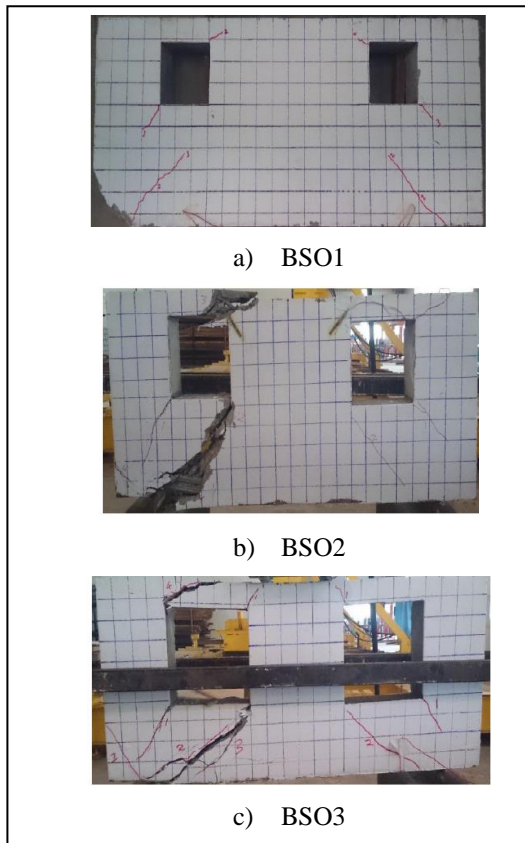
Fig. 8. Crack pattern of RC deep beams with square openings (a) BSO1 (b) BSO2, (c) BSO3
