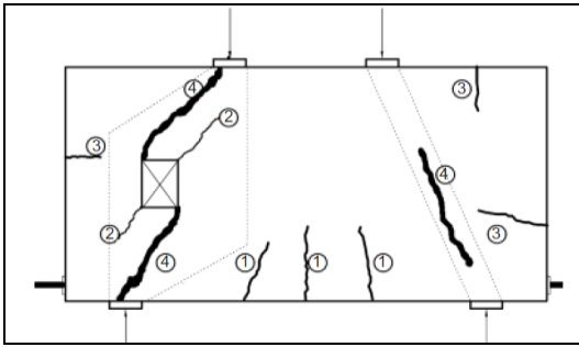
Fig. 2. Typical cracks in deep beam [5], [6]
